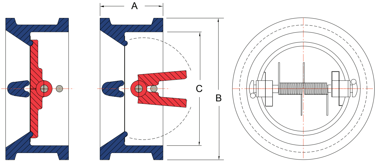
VALVE IN CLOSED POSITION
